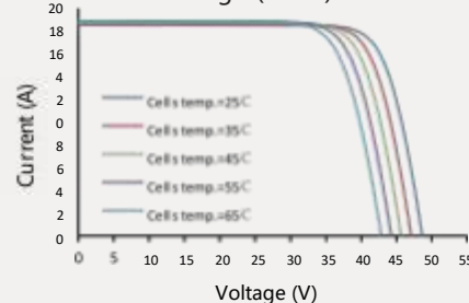
Current-Voltage (710W)
